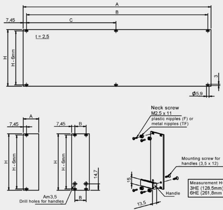
Dimensions, F and TF series
