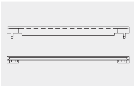
Examples for 19-plug-in modules with mounted card or cassettes guide bars.
